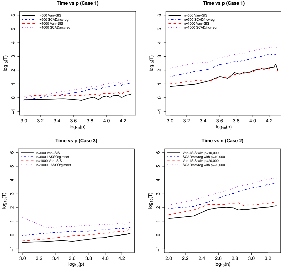
Figure 1: Median run time in seconds taken over 10 trials (log-log scale).
